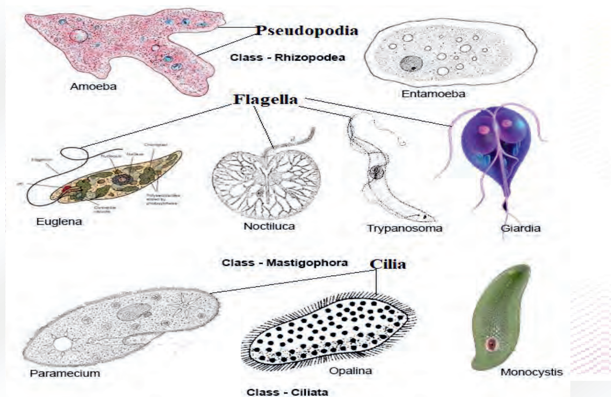
Figure 2.19. Common protozoa
