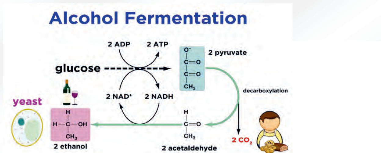
Figure 3.22. Alcohol fermentation
