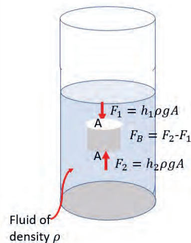
Figure 3.20 Pressure variation with depth resulting a buoyant force
