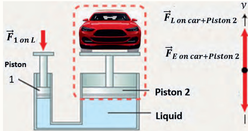
Figure 3.14 Hydraulic press
