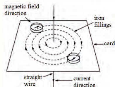
Figure 4.8 The magnetic field around a straight line.
