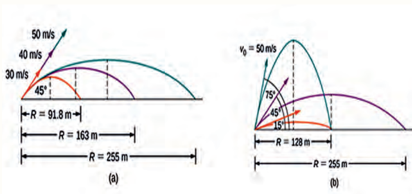
Figure 2.5 Trajectories of projectiles on leveled ground. (a) The effect of initial velocity v_0 on the range of a projectile with a given initial angle. (b) The effect of initial angle \theta on the range of a projectile with a given initial speed.
