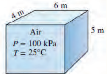
Figure 3.10 Dimension of air at 25°C and 100 kPa
