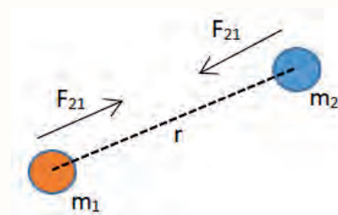
Figure 2.22 Gravitational attraction is along a line joining the centers of mass of the two bodies.
