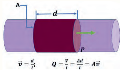
Figure 3.24 Flow rate of fluid.
