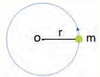
Figure 2.16 Point mass rotating about O
