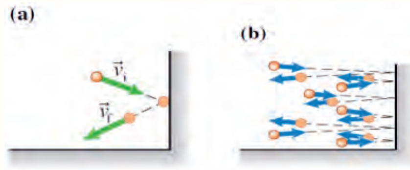
Figure 3.6 a) Each particle exerts an impulsive force on the wall (b) collective collision of gas particles on a wall.
