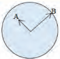
Figure 2.13 Particle A and B on the rotating disk are at different radius.
