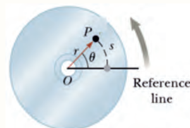
Figure 2.8 A CD rotating about a fixed axis through O perpendicular to the plane of the figure.
