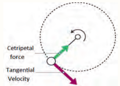
Figure 2.23 Centripetal force constantly pulls the object towards the center of the circle.
