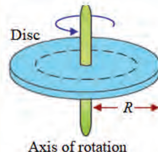
Figure 2.7 Rotation of a disc of mass M around a fixed axis.
