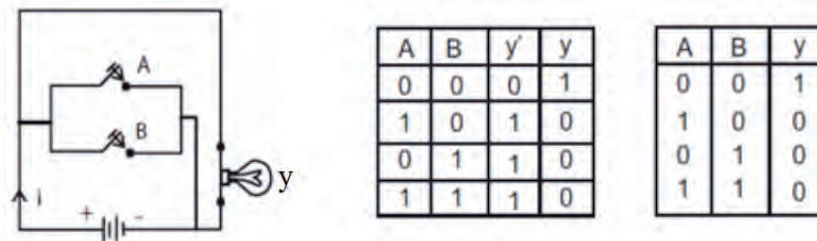
Figure 5.29 The NOR gate switch circuit and truth table.
