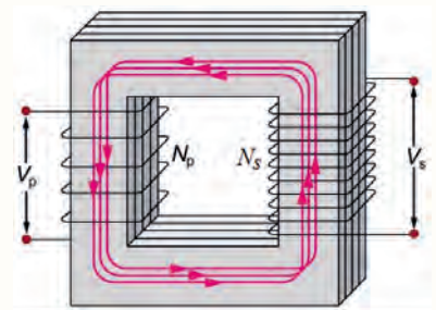
Figure 4.13 Transformer.
