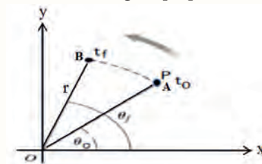
Figure 2.9 A particle P on a rotating disc moves from A to B along the arc of a circle.
