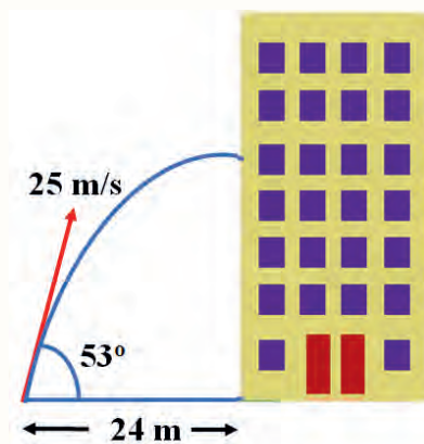
Figure 2.6 A ball thrown toward a wall.
